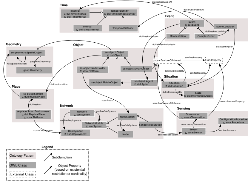
Fig. 1. SmartEnv Ontology is composed of 8 ontology patterns.
